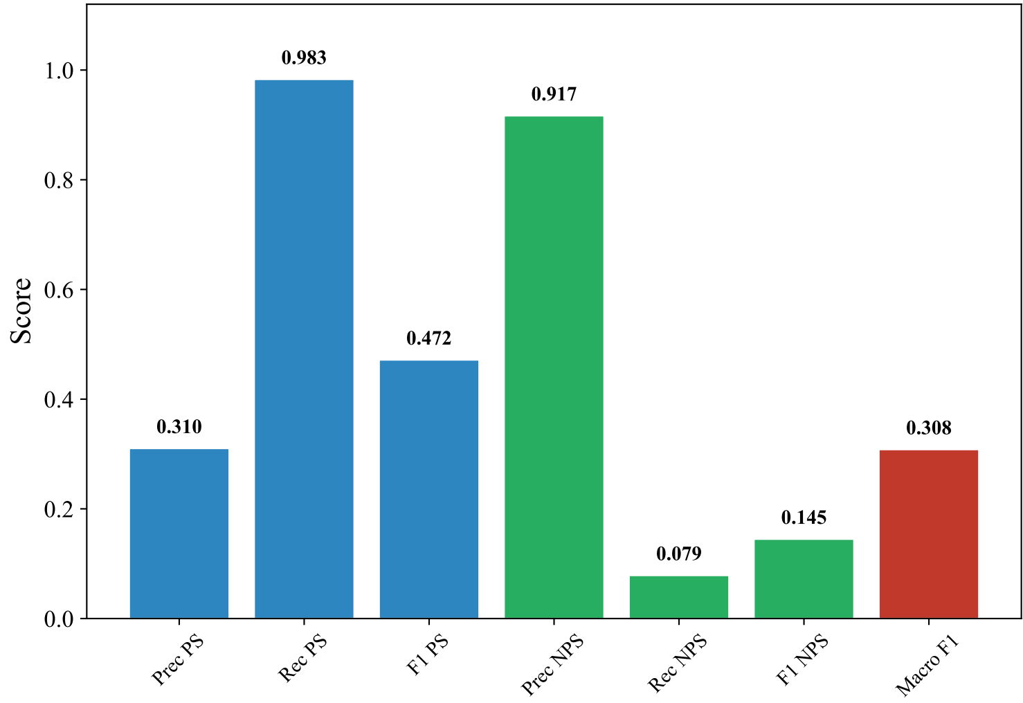
Classification Metrics — DUTCH_MANUAL (snowflake-arctic-embed-l-v2.0, lightgbm)
