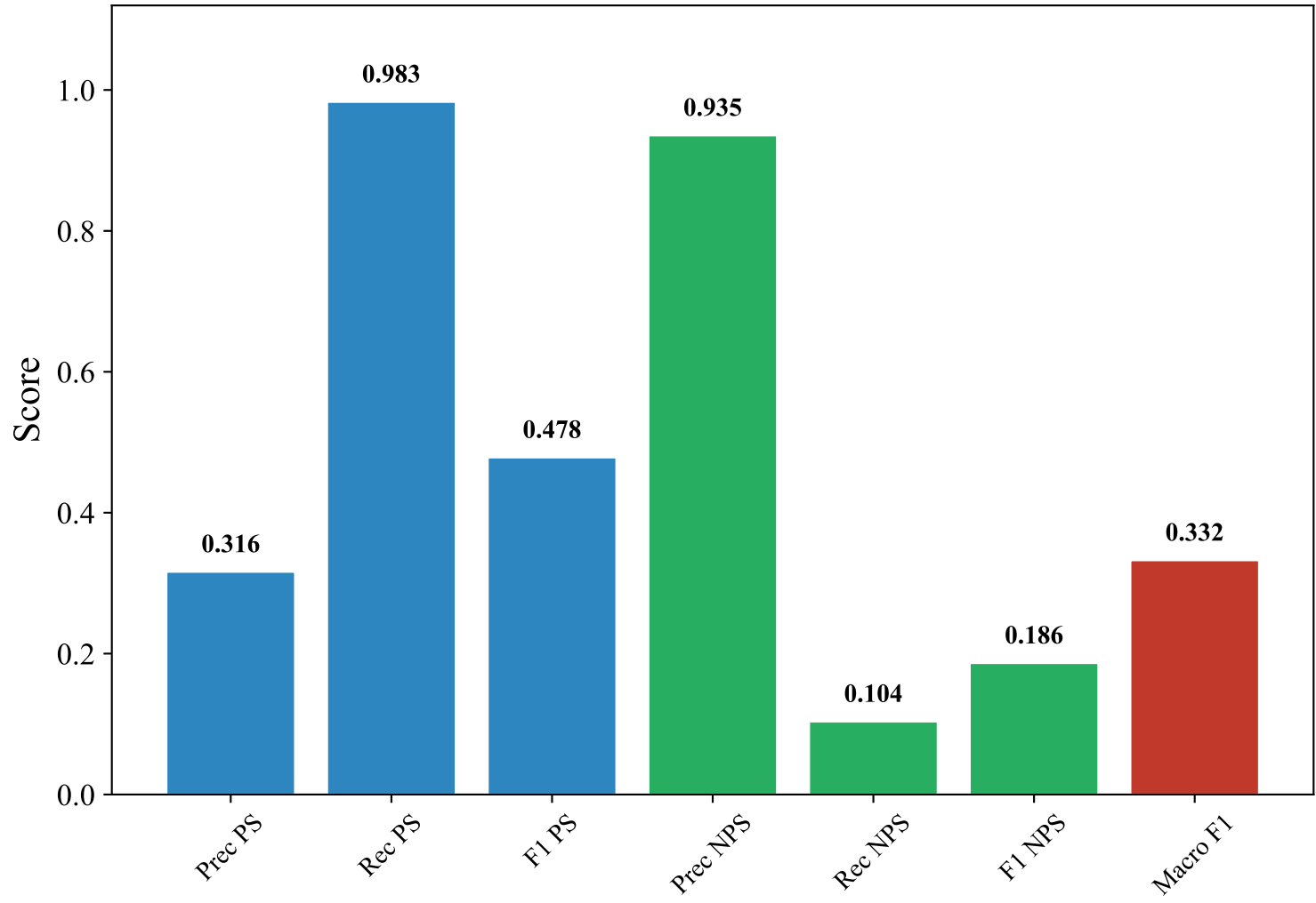
Classification Metrics — DUTCH_MANUAL (snowflake-arctic-embed-l-v2.0, svm_linear)
