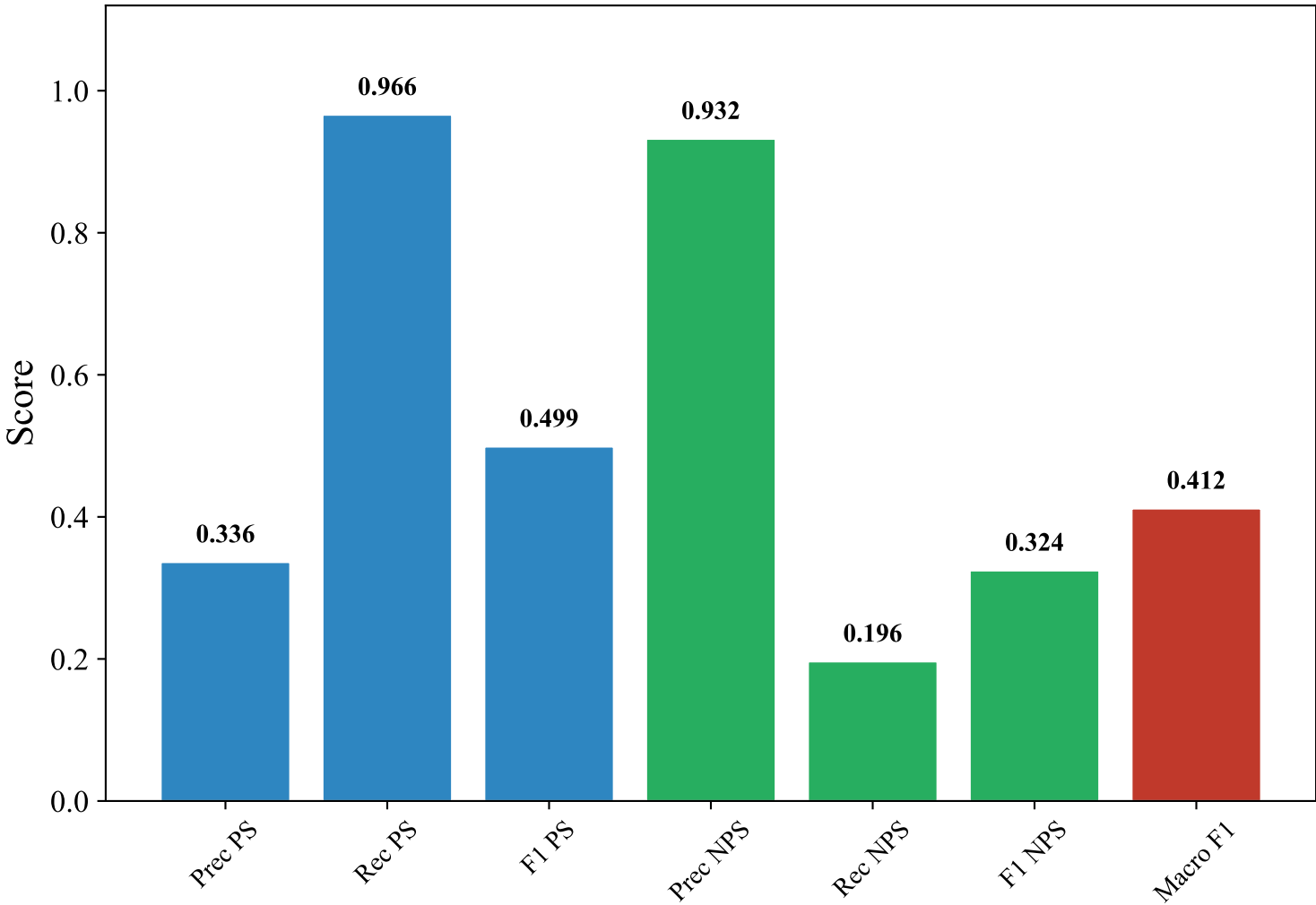
Classification Metrics — DUTCH_MANUAL (xlm-roberta-base, svm_linear)
