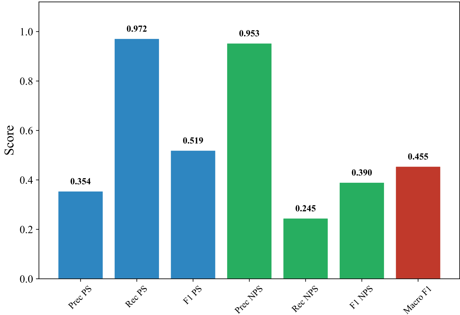
Classification Metrics — ENGLISH_MANUAL (bert-base-multilingual-uncased, svm_linear)
