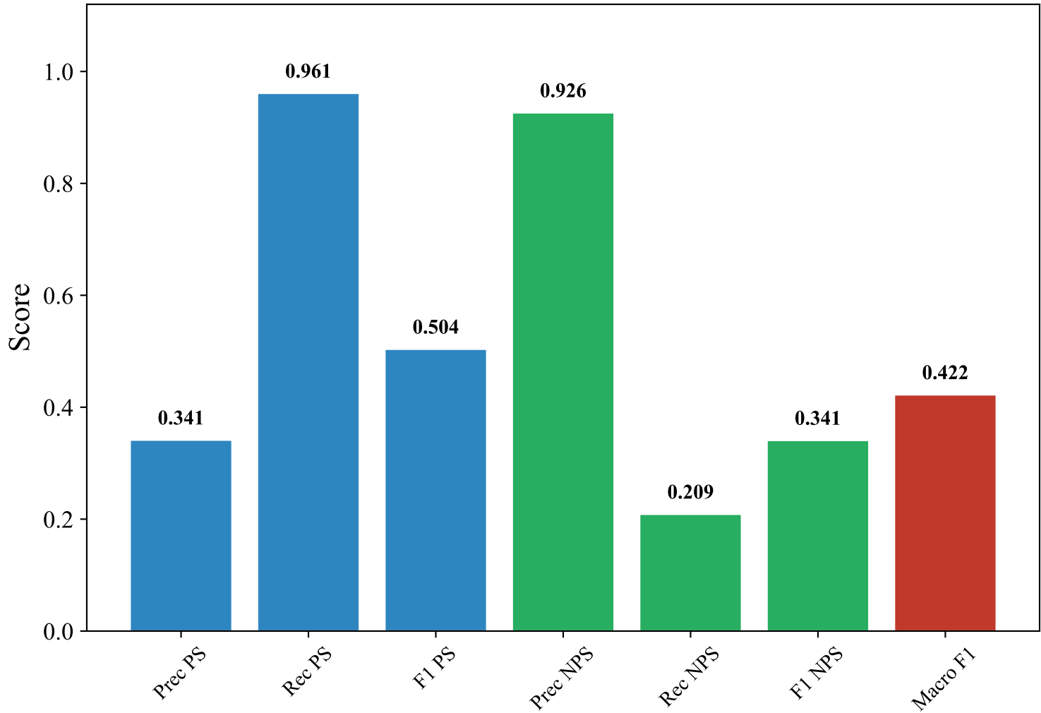
Classification Metrics — ENGLISH_MANUAL (multilingual-e5-large-instruct, random_forest)
