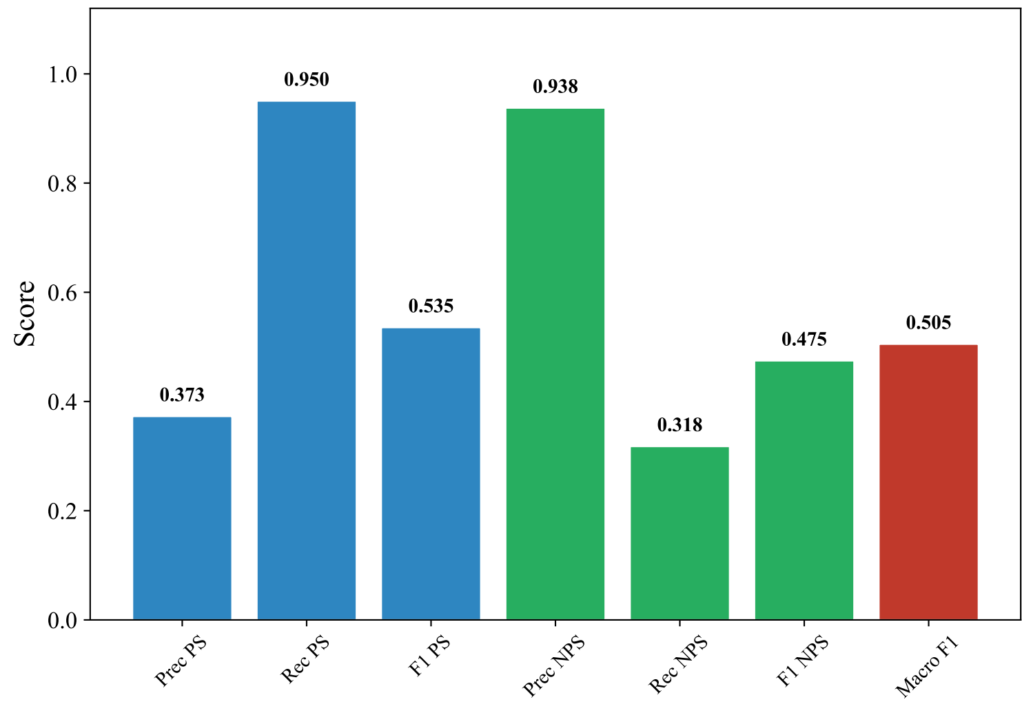
Classification Metrics — ENGLISH_MANUAL (multilingual-e5-large-instruct, svm_linear)
