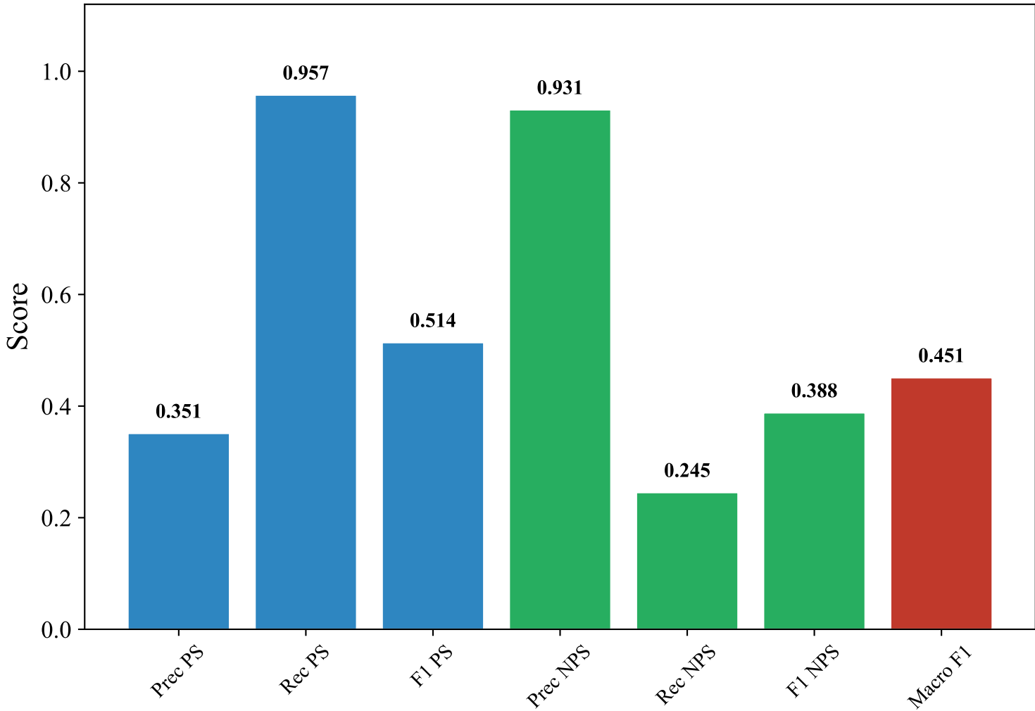
Classification Metrics — ENGLISH_MANUAL (multilingual-e5-large-instruct, xgboost)
