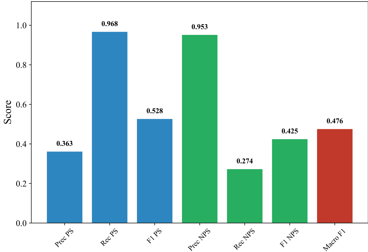
Classification Metrics — ENGLISH_MANUAL (paraphrase-multilingual-MiniLM-L12-v2, svm_rbf)
