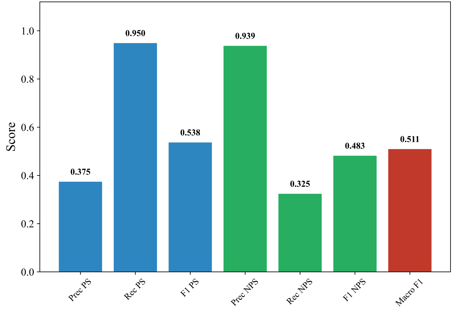
Classification Metrics — ENGLISH_MANUAL (paraphrase-multilingual-MiniLM-L12-v2, xgboost)
