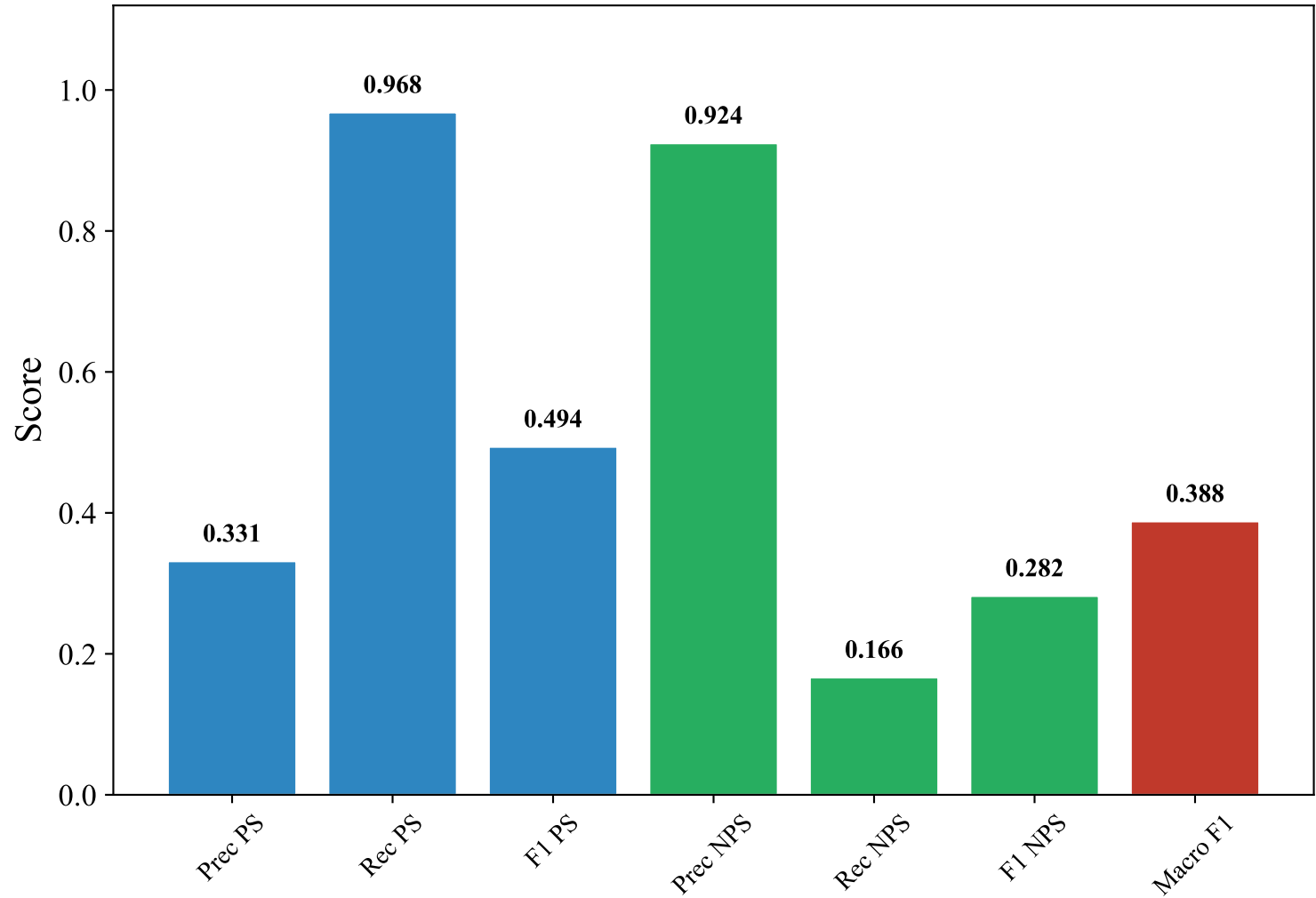
Classification Metrics — ENGLISH_MANUAL (snowflake-arctic-embed-l-v2.0, random_forest)
