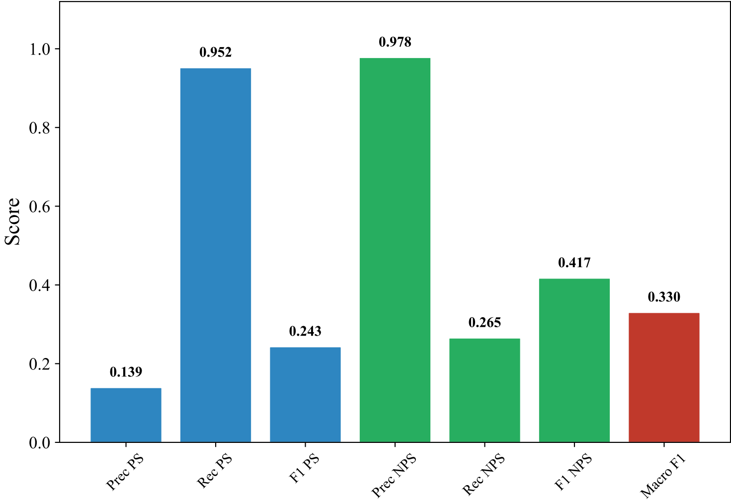
Classification Metrics — GERMAN_MANUAL (bert-base-multilingual-uncased, random_forest)
