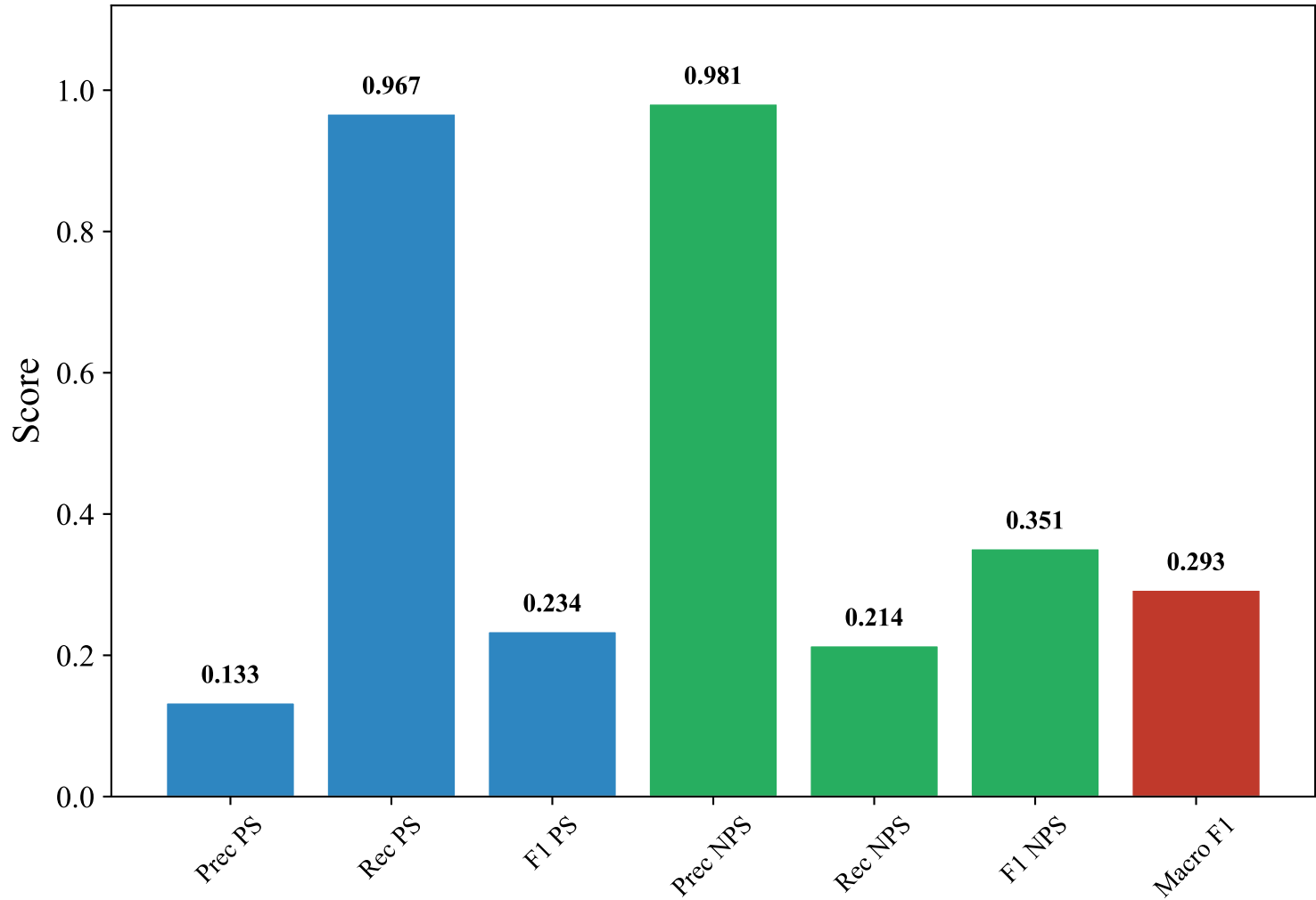
Classification Metrics — GERMAN_MANUAL (bert-base-multilingual-uncased, svm_linear)
