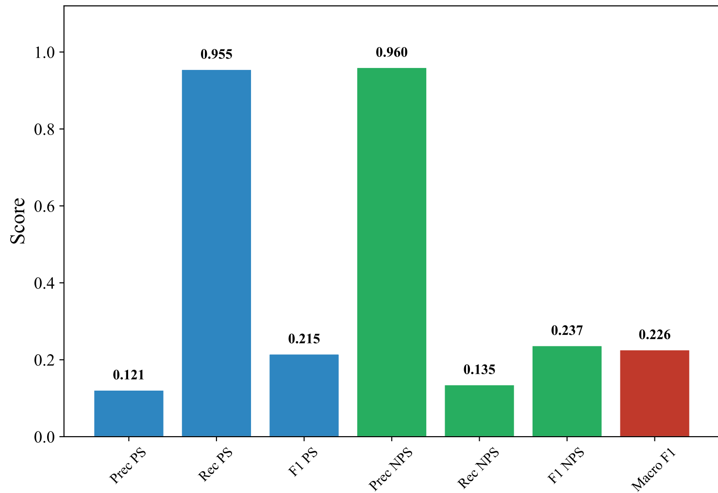
Classification Metrics — GERMAN_MANUAL (paraphrase-multilingual-MiniLM-L12-v2, random_forest)
