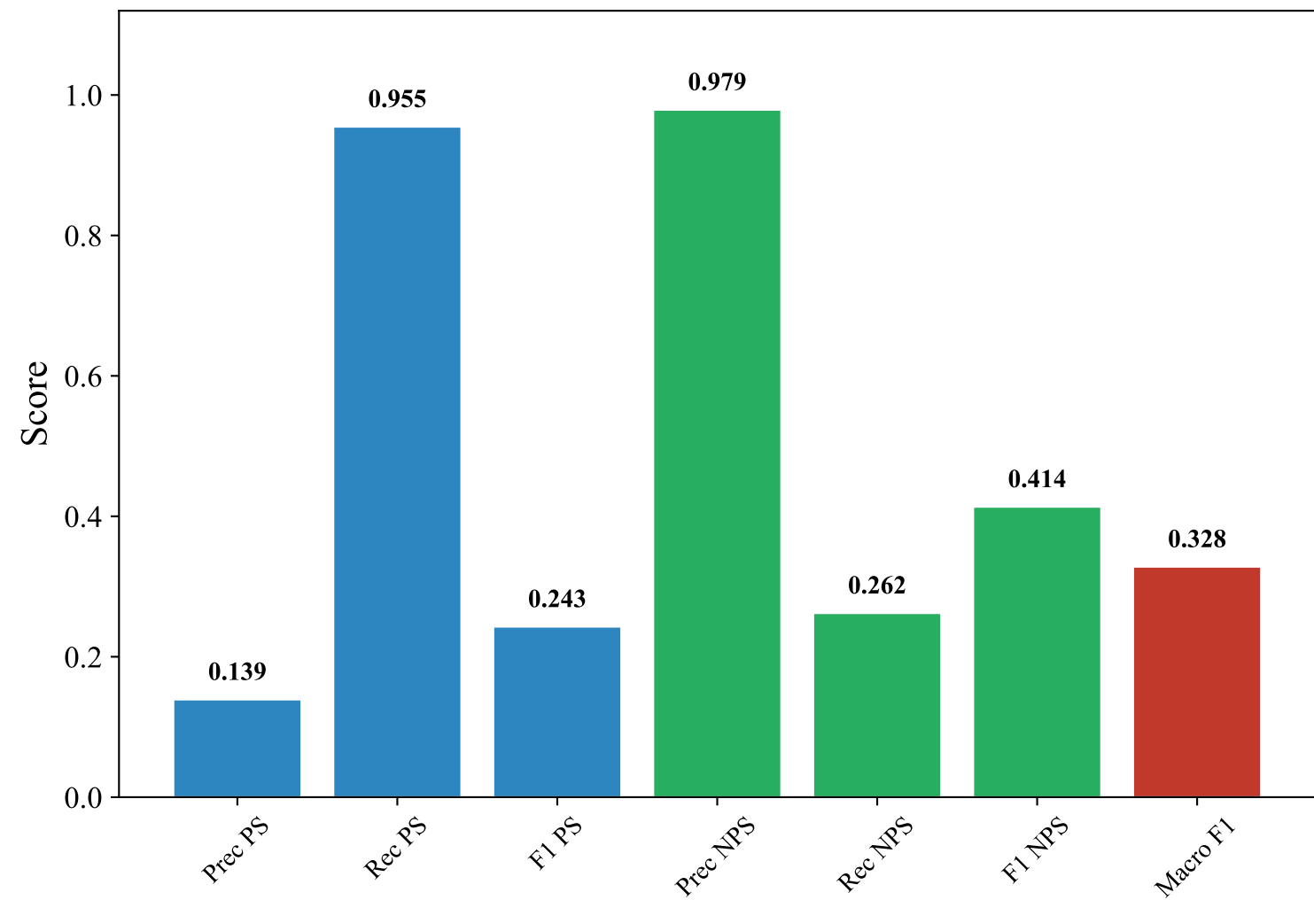
Classification Metrics — GERMAN_MANUAL (paraphrase-multilingual-mpnet-base-v2, svm_rbf)
