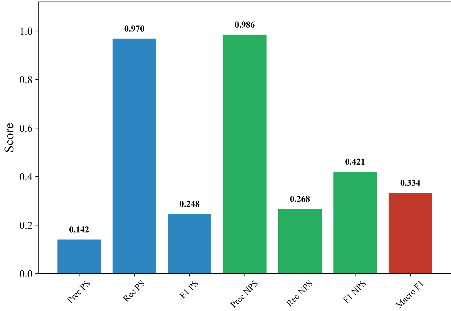
Classification Metrics — GERMAN_MANUAL (snowflake-arctic-embed-l-v2.0, svm_linear)
