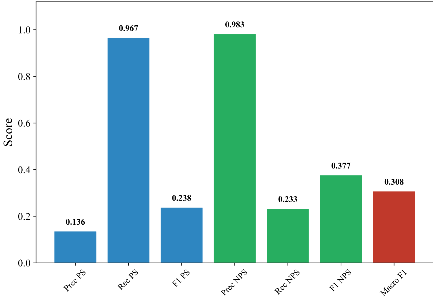
Classification Metrics — GERMAN_MANUAL (xlm-roberta-base, svm_linear)
