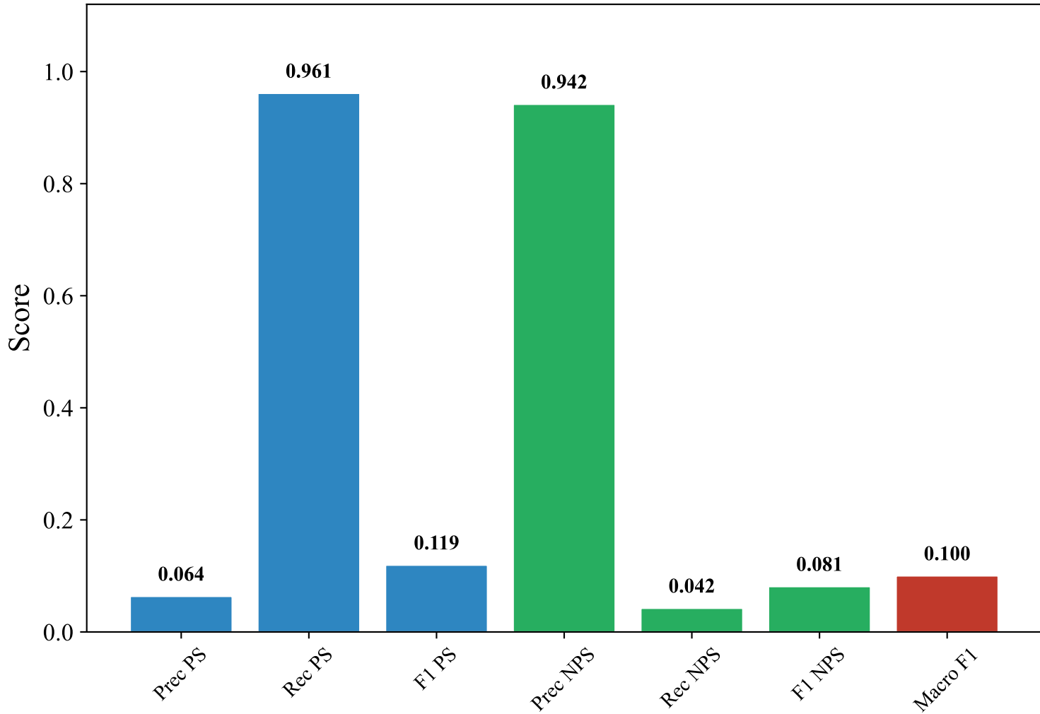
Classification Metrics — SWEDISH_MANUAL (bert-base-multilingual-uncased, svm_rbf)
