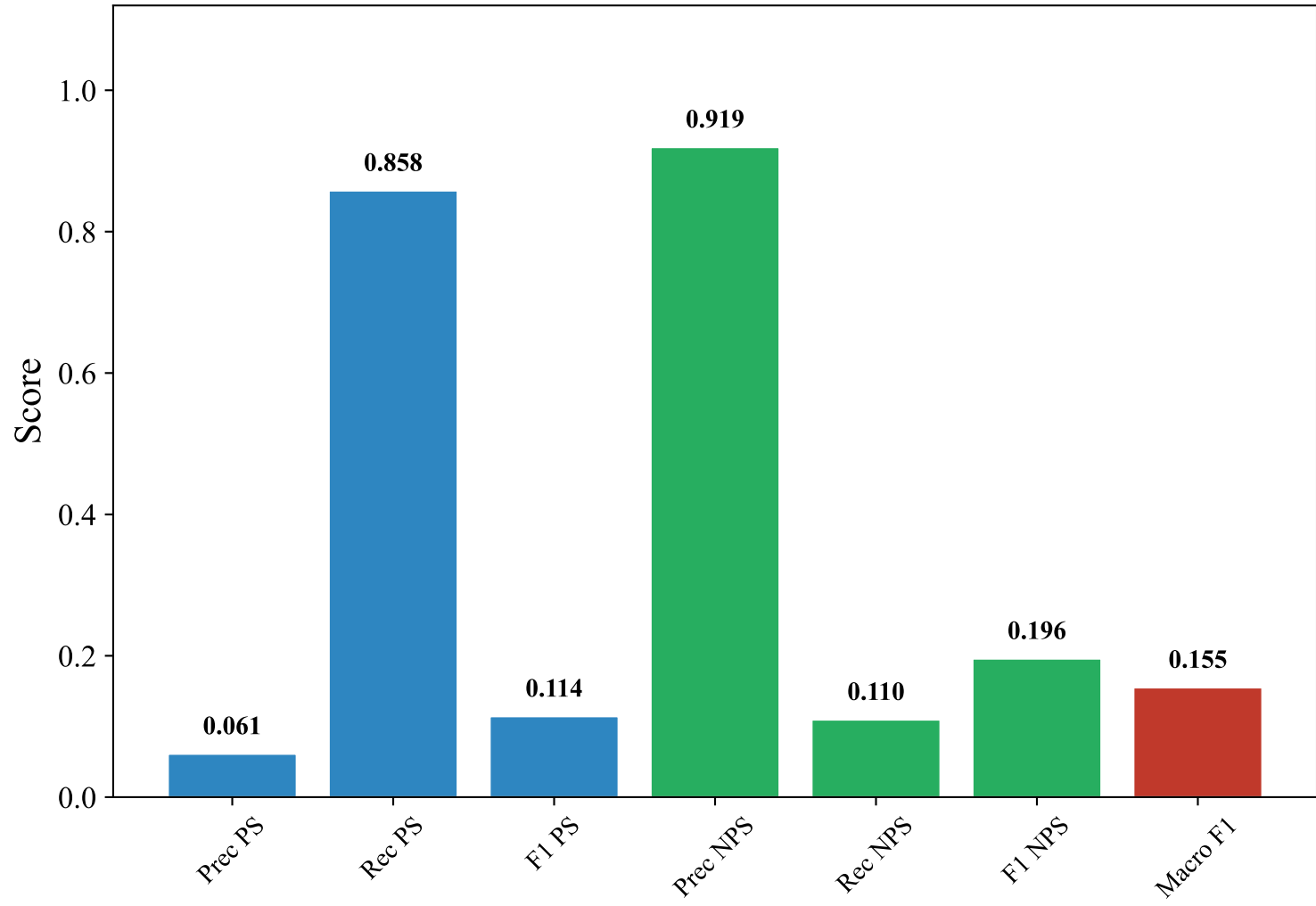
Classification Metrics — SWEDISH_MANUAL (bert-base-multilingual-uncased, xgboost)
