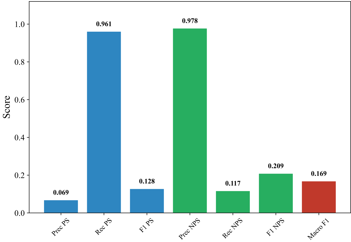
Classification Metrics — SWEDISH_MANUAL (multilingual-e5-large-instruct, svm_linear)
