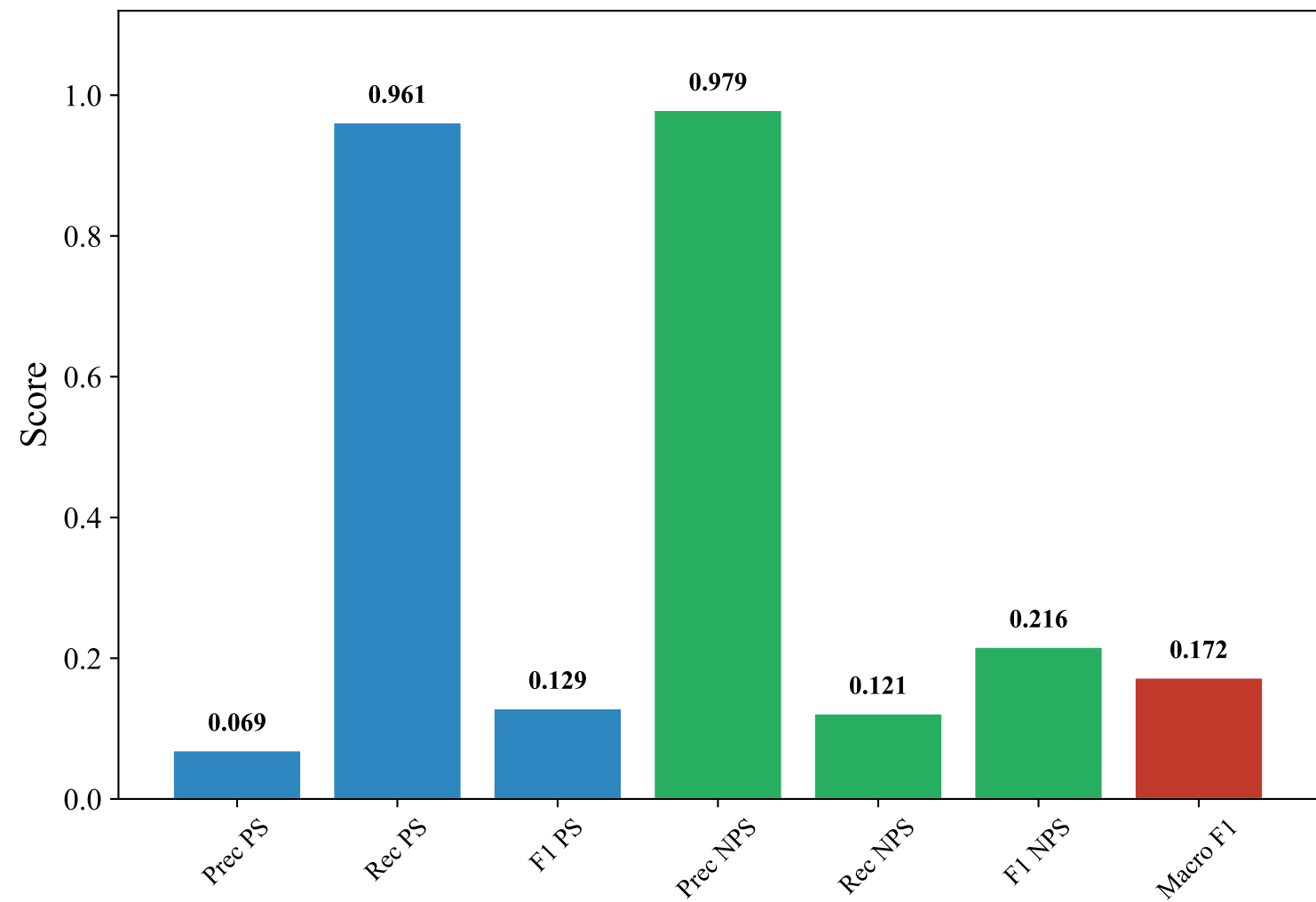
Classification Metrics — SWEDISH_MANUAL (paraphrase-multilingual-MiniLM-L12-v2, random_forest)
