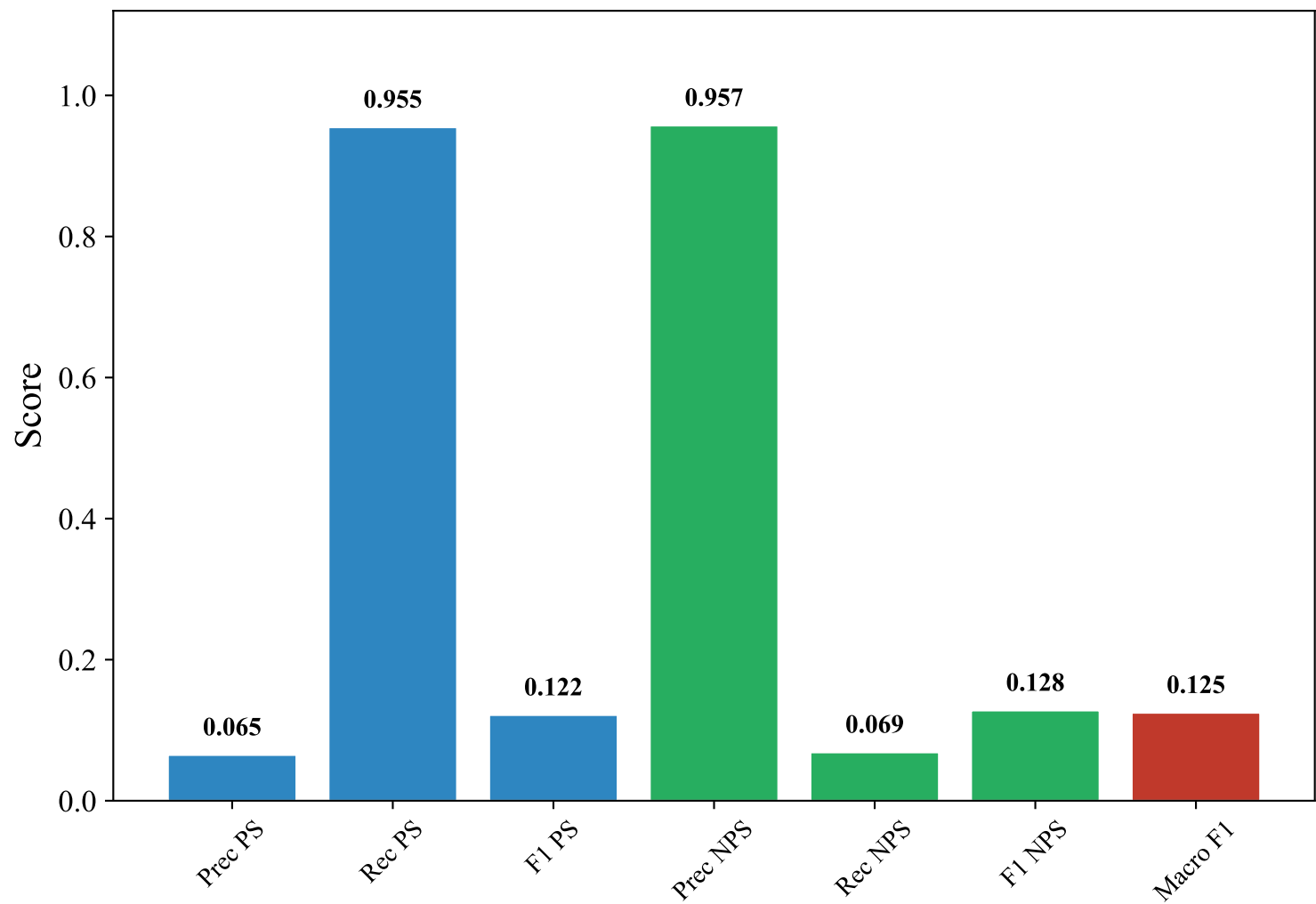
Classification Metrics — SWEDISH_MANUAL (paraphrase-multilingual-MiniLM-L12-v2, svm_rbf)
