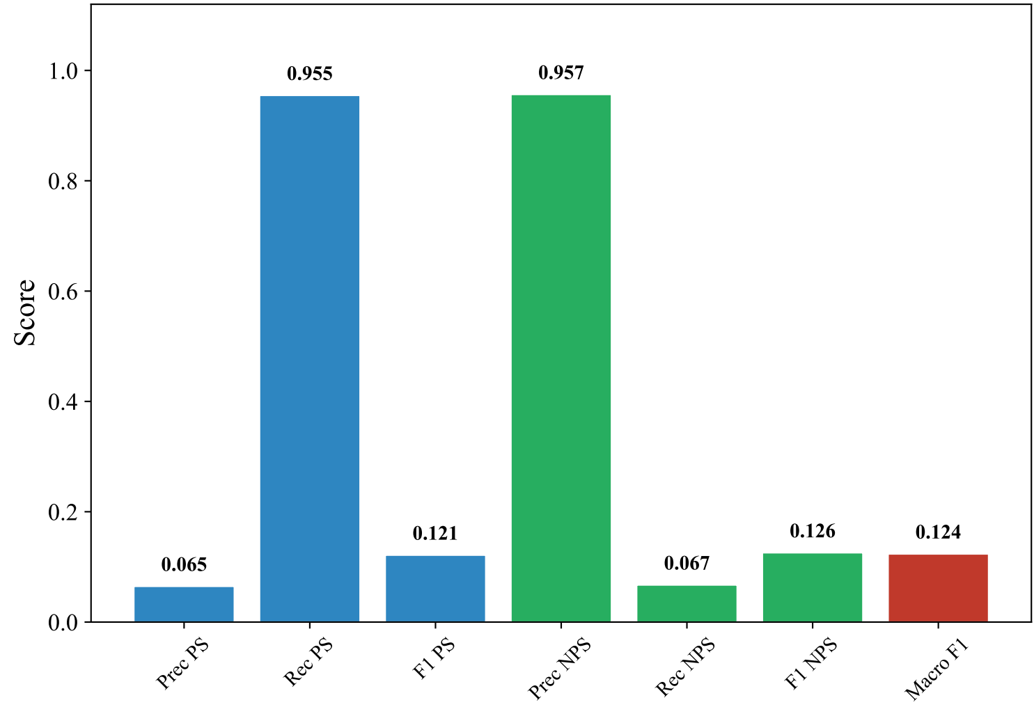
Classification Metrics — SWEDISH_MANUAL (paraphrase-multilingual-mpnet-base-v2, lightgbm)
