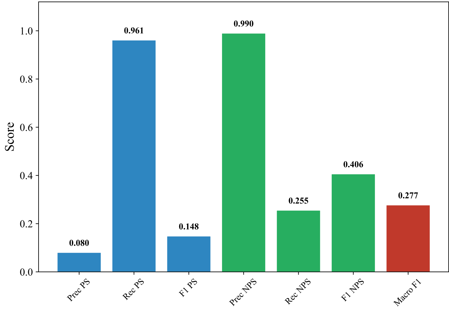
Classification Metrics — SWEDISH_MANUAL (snowflake-arctic-embed-l-v2.0, svm_linear)
