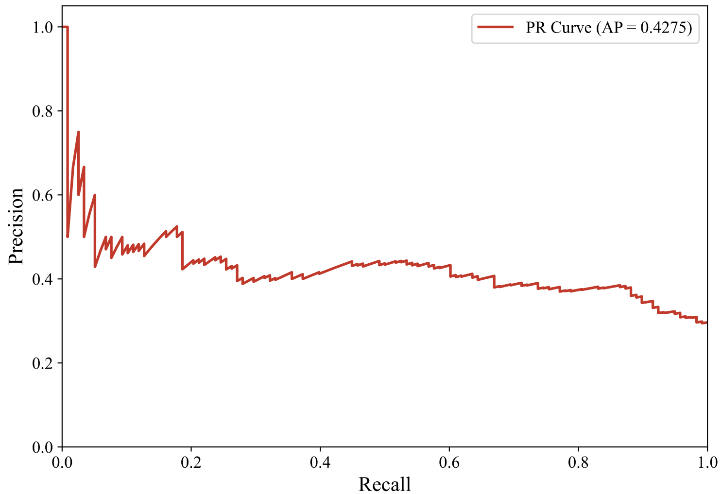
Precision-Recall Curve — DUTCH_MANUAL (bert-base-multilingual-uncased, svm_linear)
