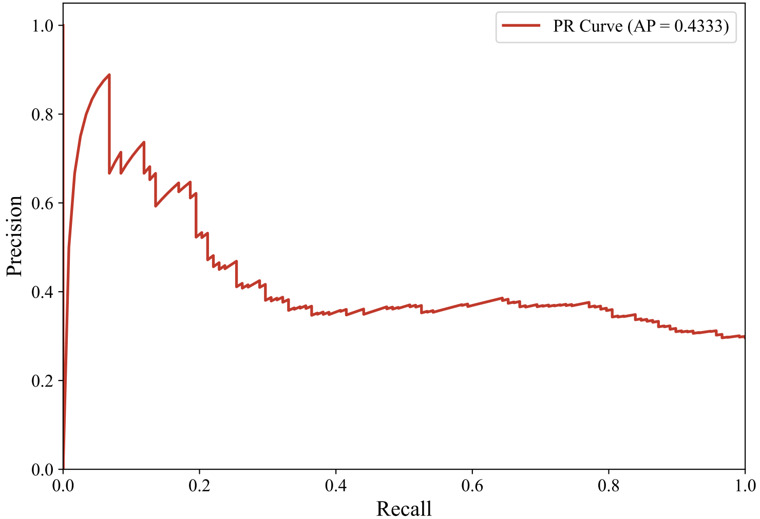
Precision-Recall Curve — DUTCH_MANUAL (bert-base-multilingual-uncased, svm_rbf)
