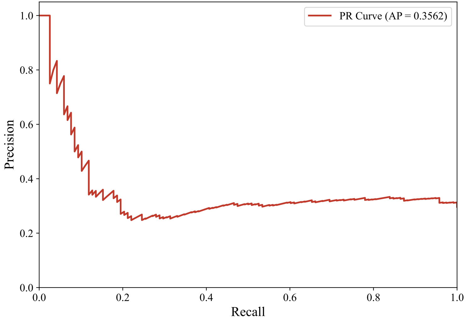
Precision-Recall Curve — DUTCH_MANUAL (multilingual-e5-large-instruct, lightgbm)
