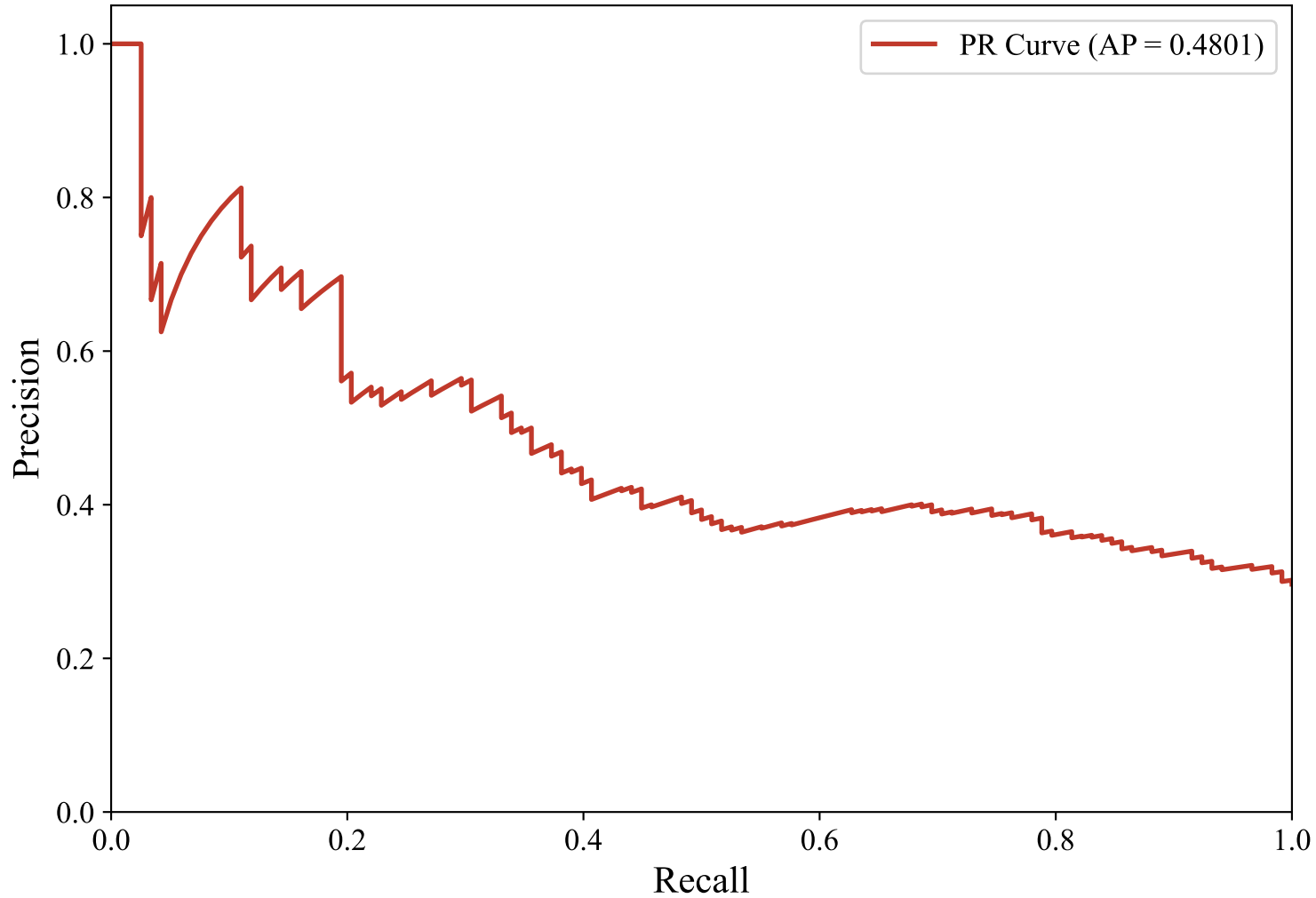
Precision-Recall Curve — DUTCH_MANUAL (multilingual-e5-large-instruct, random_forest)
