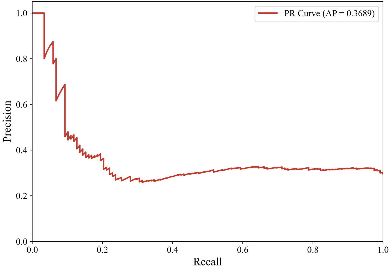
Precision-Recall Curve — DUTCH_MANUAL (multilingual-e5-large-instruct, xgboost)
