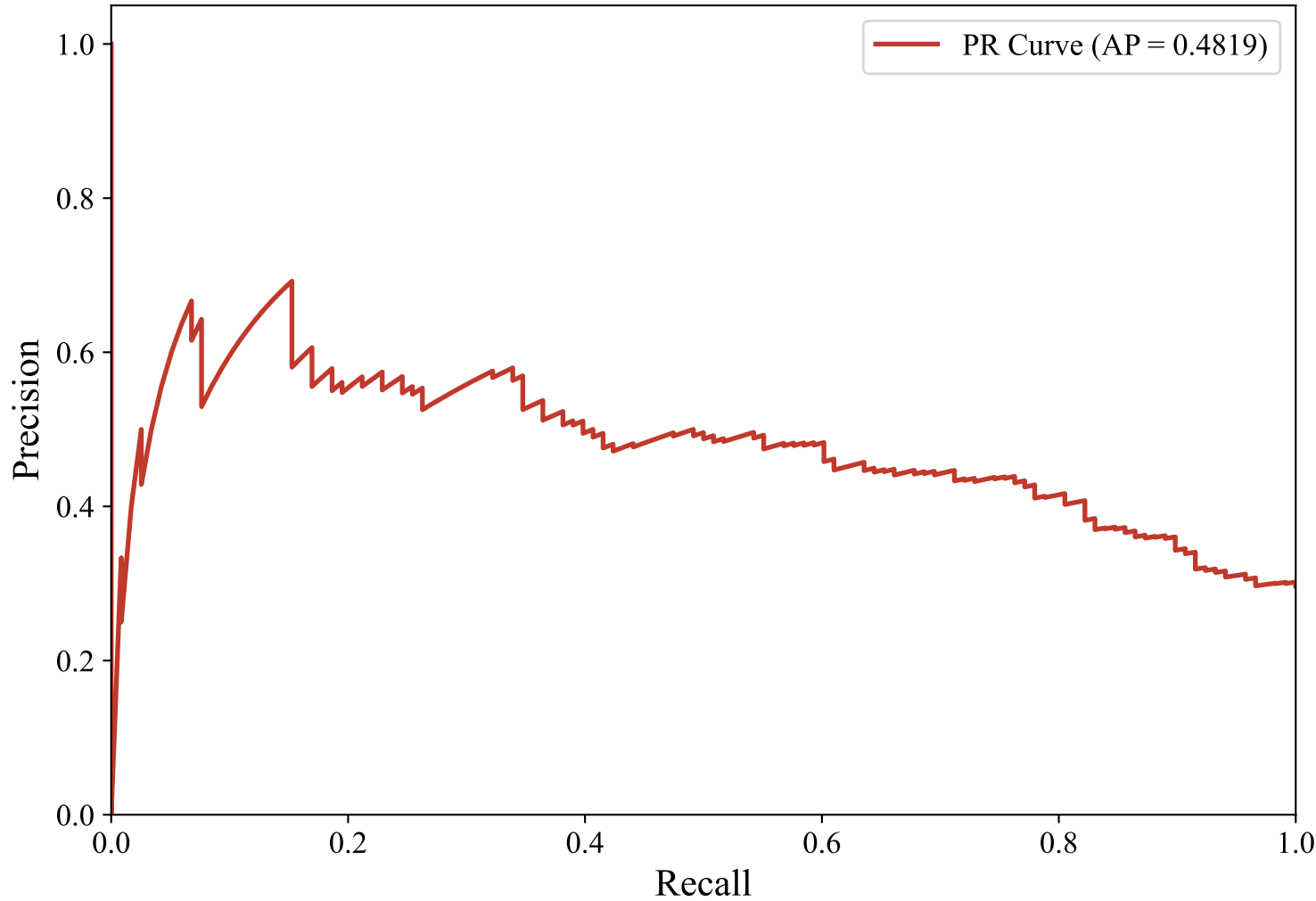
Precision-Recall Curve — DUTCH_MANUAL (paraphrase-multilingual-MiniLM-L12-v2, random_forest)
