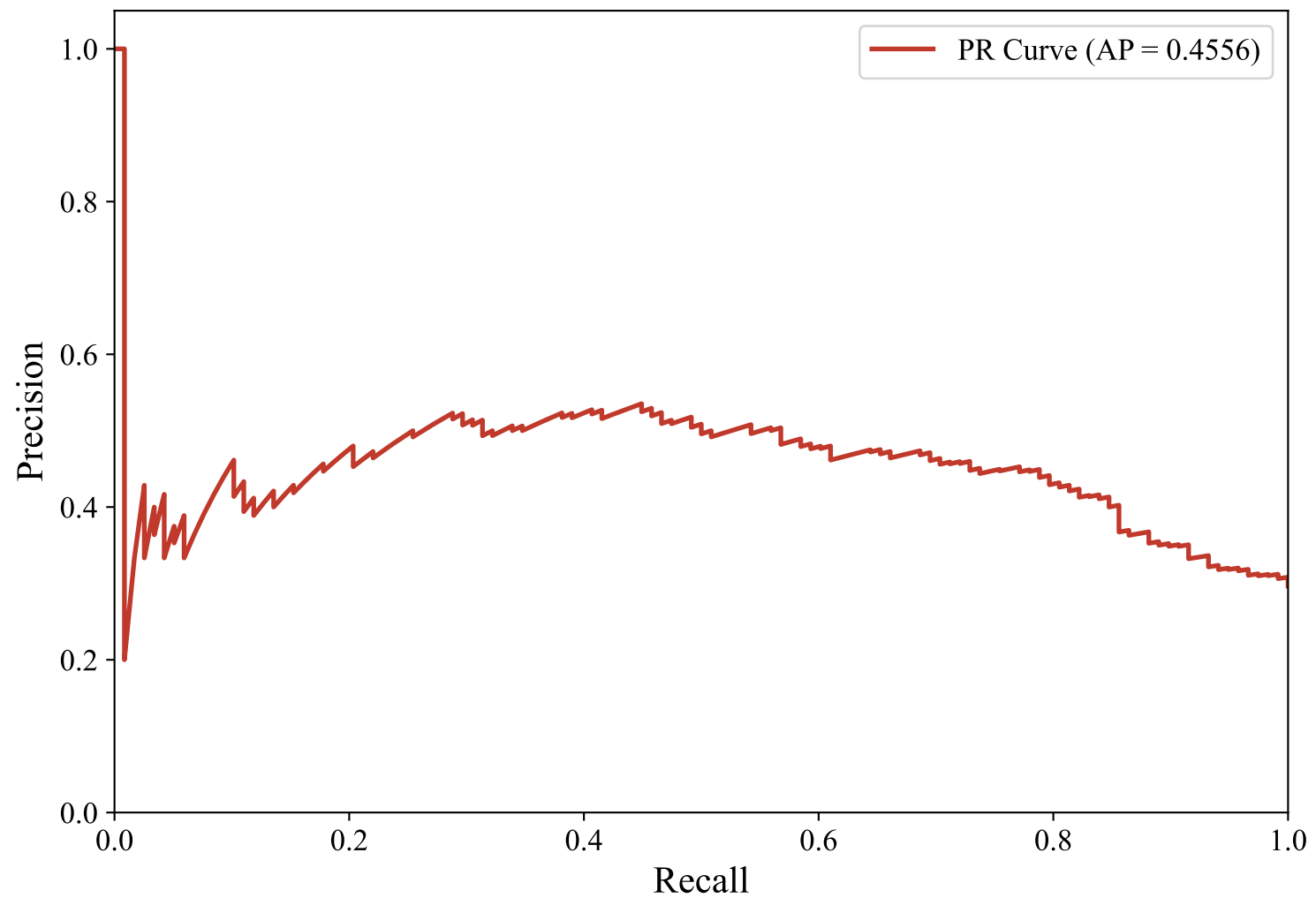
Precision-Recall Curve — DUTCH_MANUAL (paraphrase-multilingual-MiniLM-L12-v2, svm_linear)
