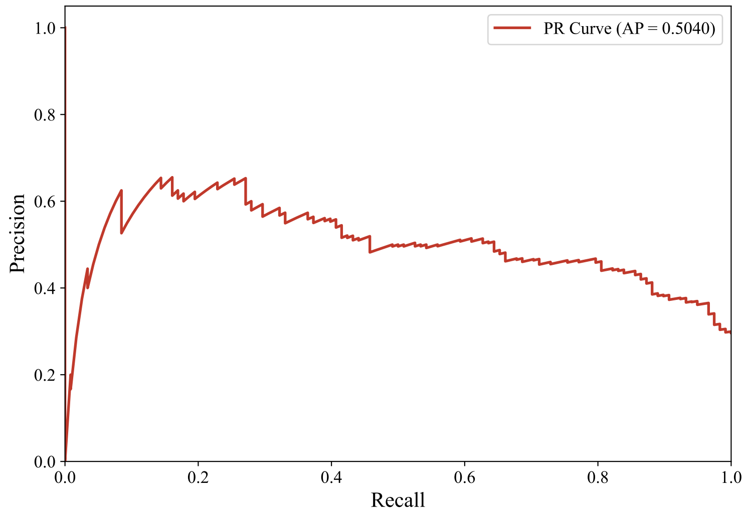
Precision-Recall Curve — DUTCH_MANUAL (paraphrase-multilingual-MiniLM-L12-v2, svm_rbf)
