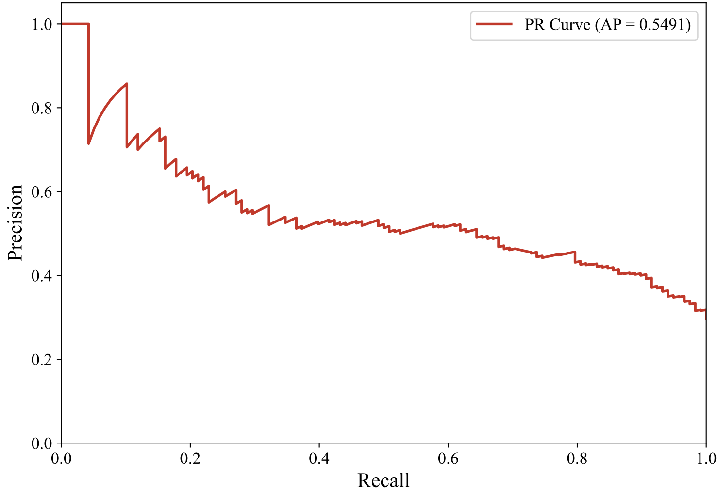
Precision-Recall Curve — DUTCH_MANUAL (paraphrase-multilingual-mpnet-base-v2, svm_rbf)
