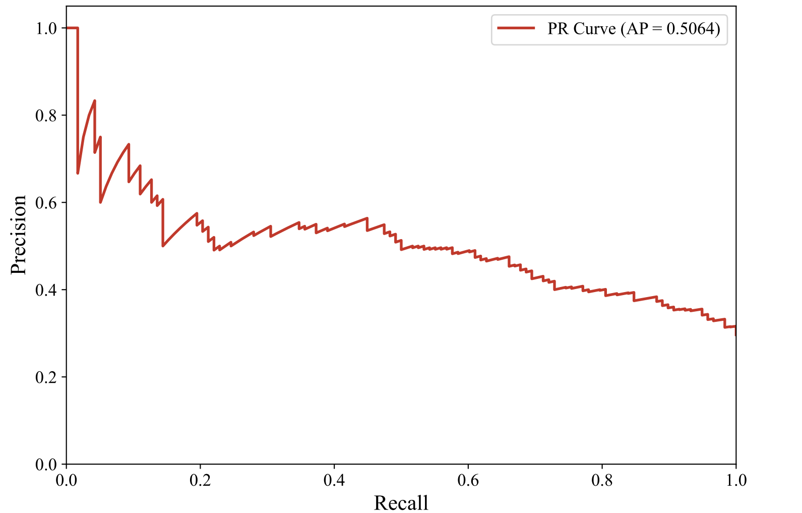
Precision-Recall Curve — DUTCH_MANUAL (paraphrase-multilingual-mpnet-base-v2, xgboost)
