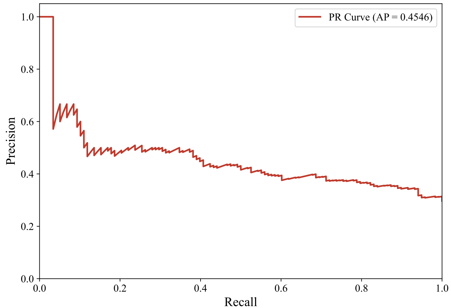
Precision-Recall Curve — DUTCH_MANUAL (snowflake-arctic-embed-l-v2.0,random_forest)
