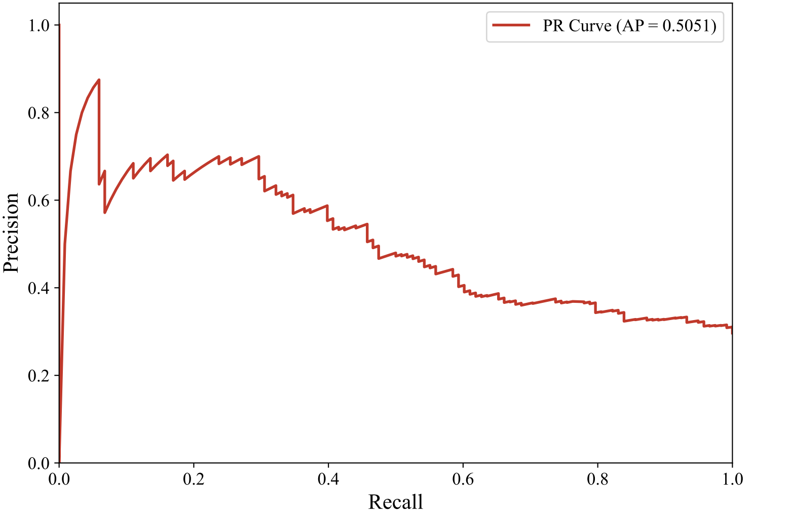
Precision-Recall Curve — DUTCH_MANUAL (xlm-roberta-base, svm_rbf)
