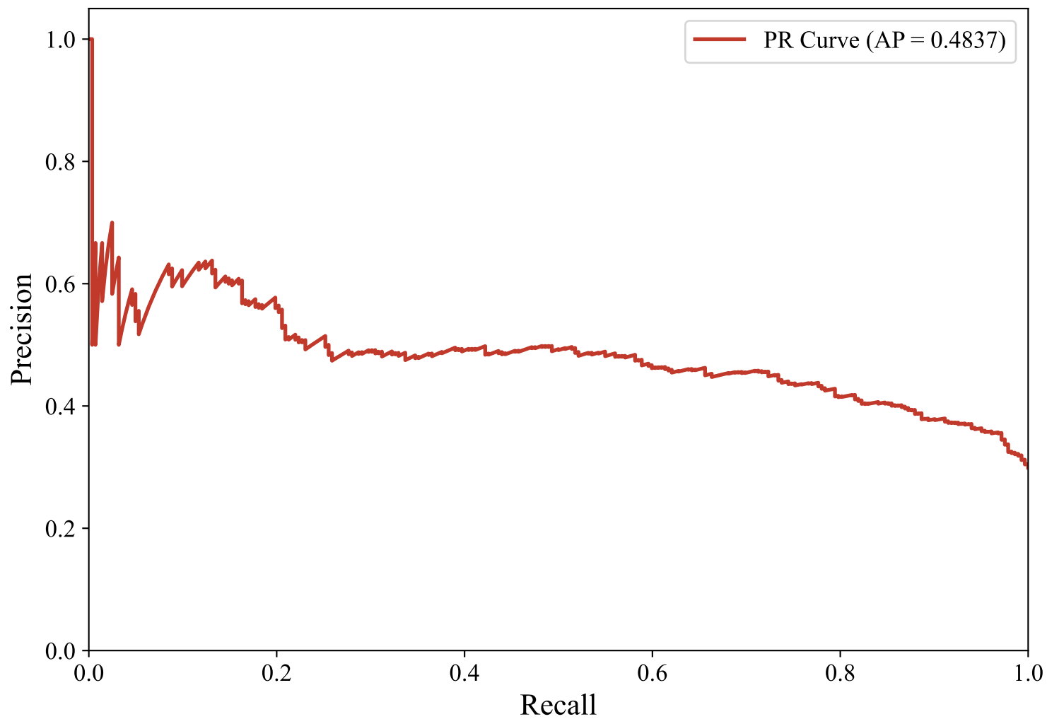
Precision-Recall Curve — ENGLISH_MANUAL (bert-base-multilingual-uncased, svm_linear)
