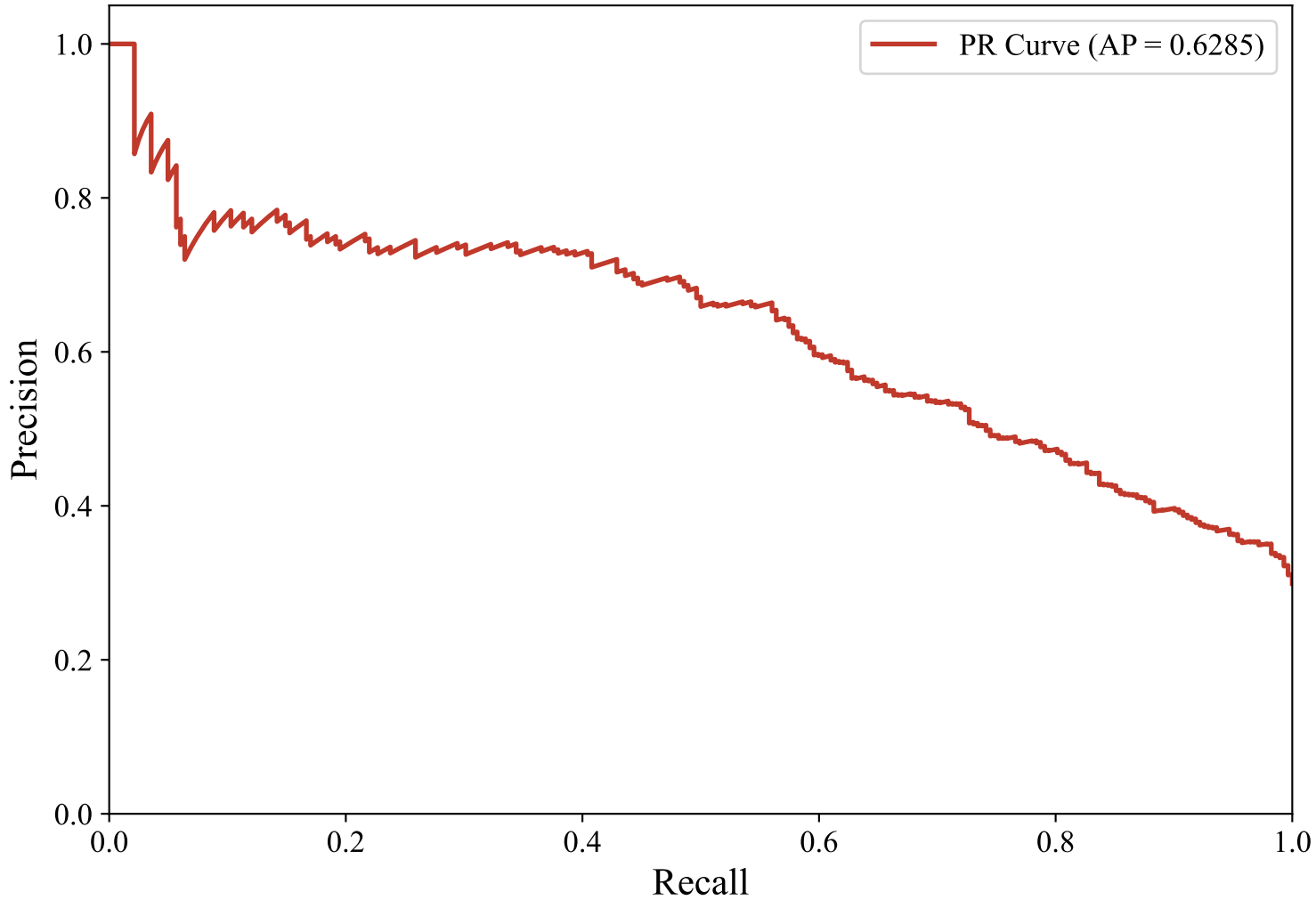
Precision-Recall Curve — ENGLISH_MANUAL (bert-base-multilingual-uncased, svm_rbf)
