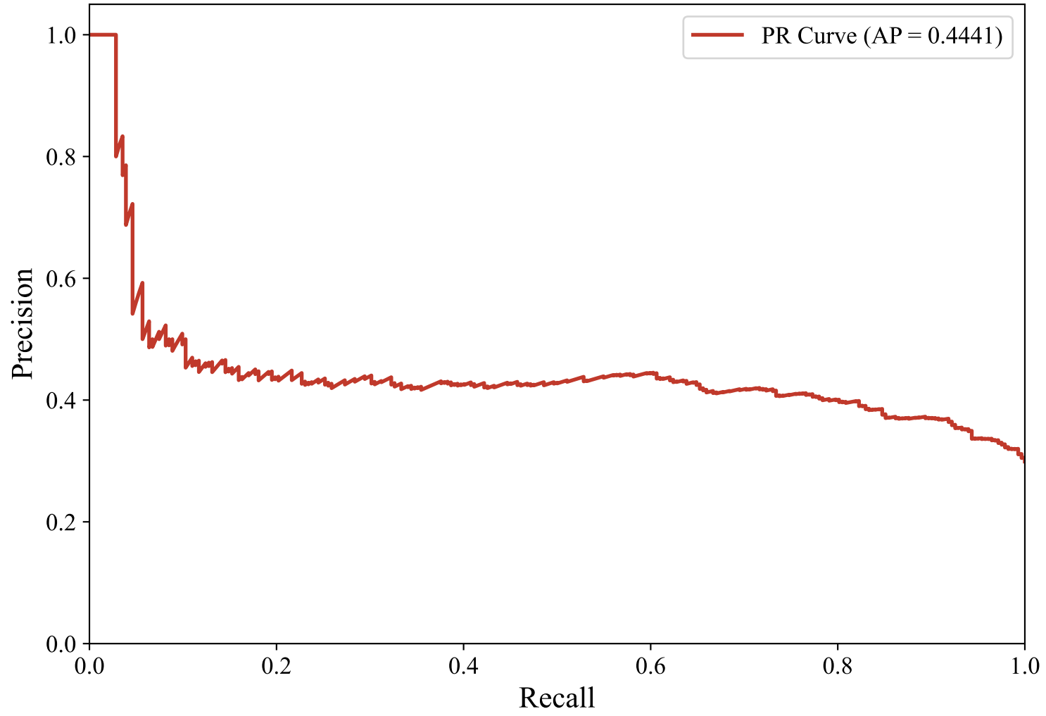
Precision-Recall Curve — ENGLISH_MANUAL (bert-base-multilingual-uncased, xgboost)
