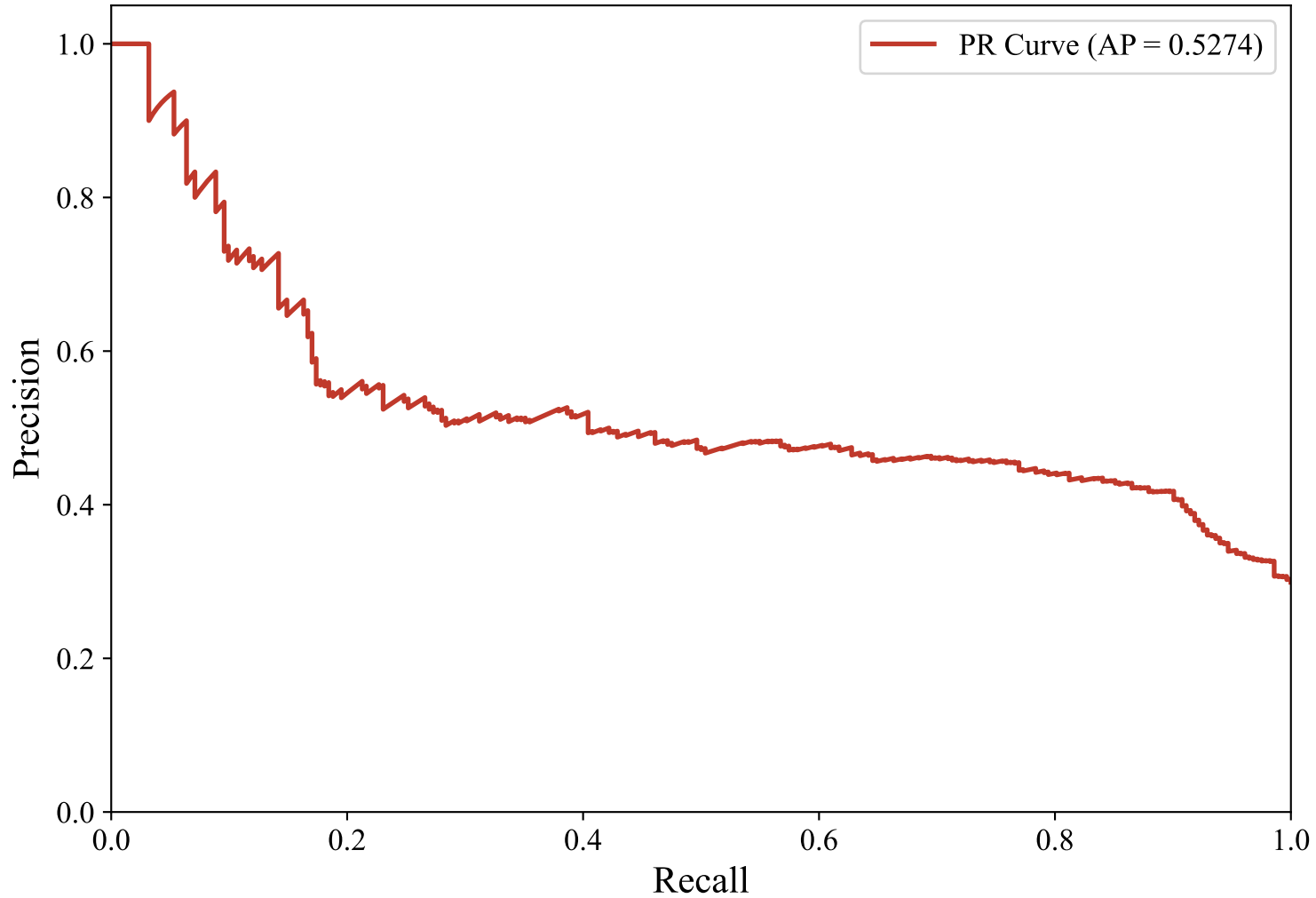
Precision-Recall Curve — ENGLISH_MANUAL (multilingual-e5-large-instruct, lightgbm)
