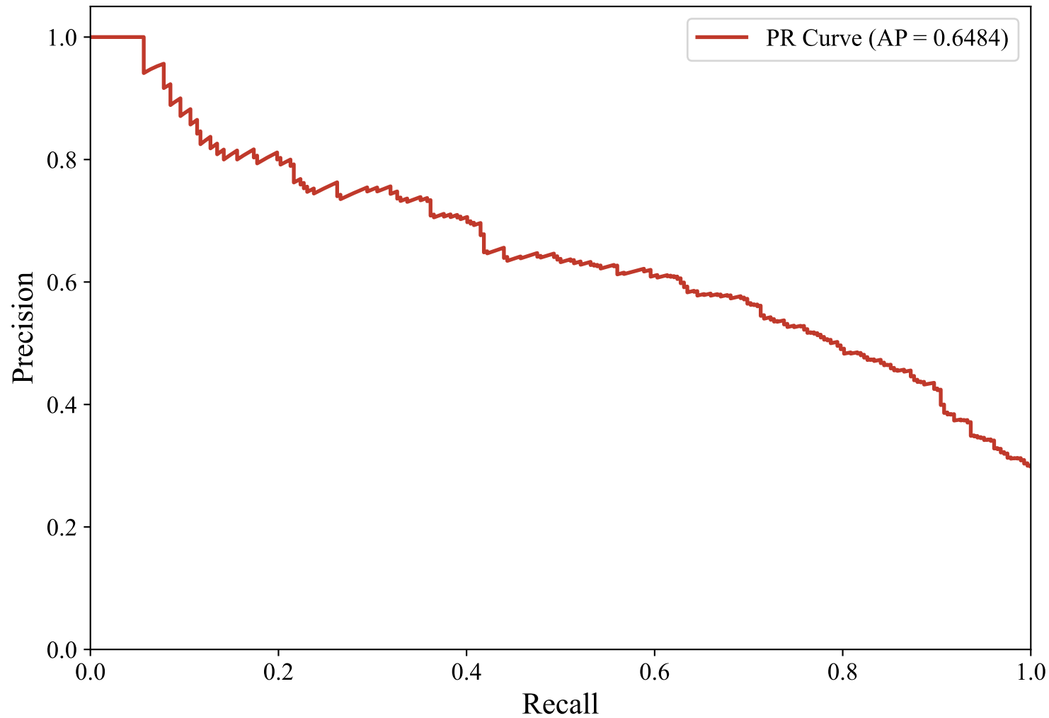
Precision-Recall Curve — ENGLISH_MANUAL (multilingual-e5-large-instruct, random_forest)
