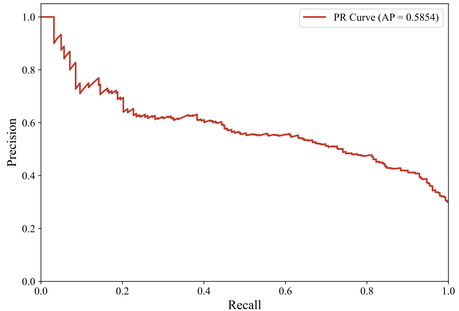
Precision-Recall Curve — ENGLISH_MANUAL (multilingual-e5-large-instruct, svm_linear)
