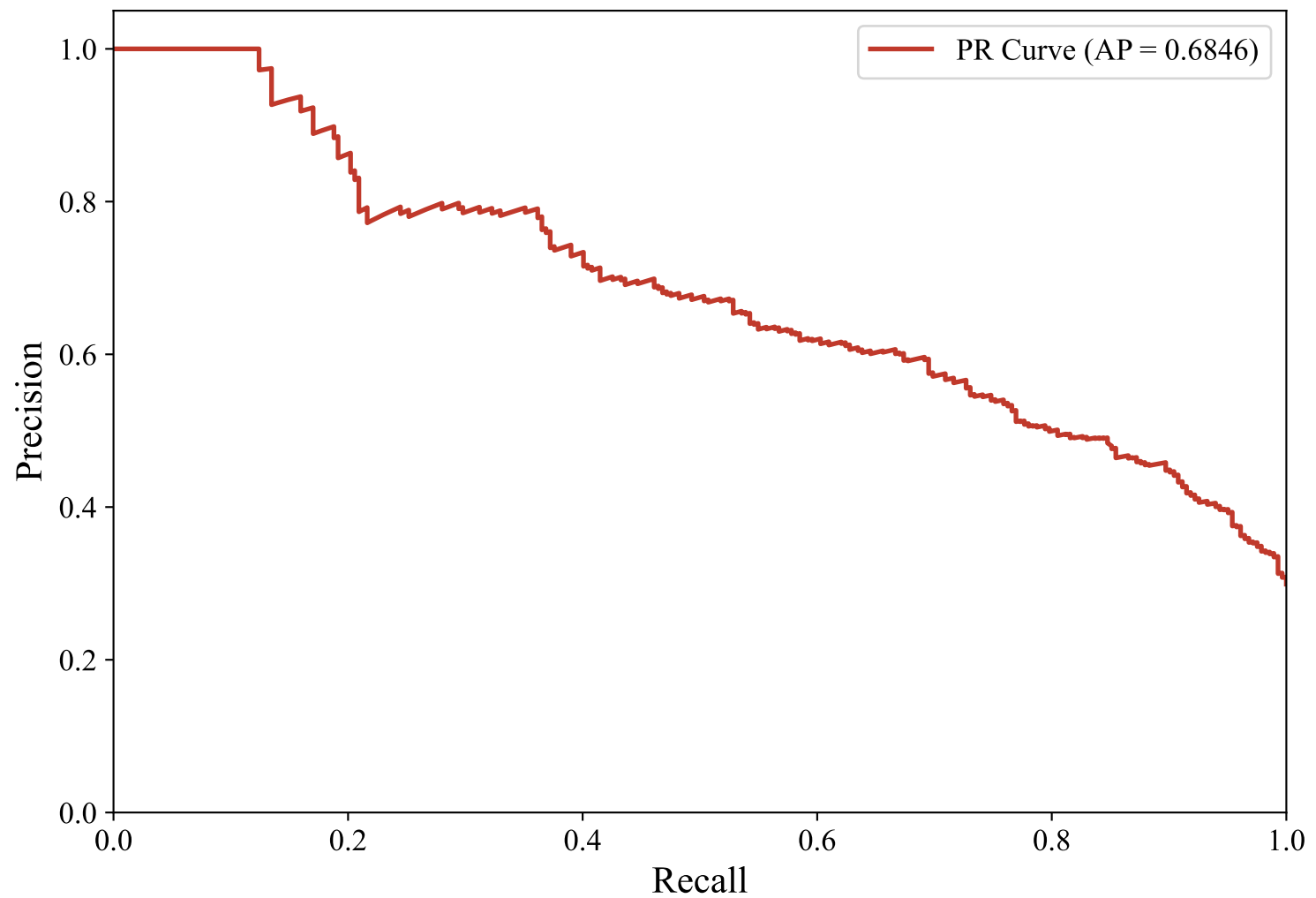
Precision-Recall Curve — ENGLISH_MANUAL (multilingual-e5-large-instruct, svm_rbf)
