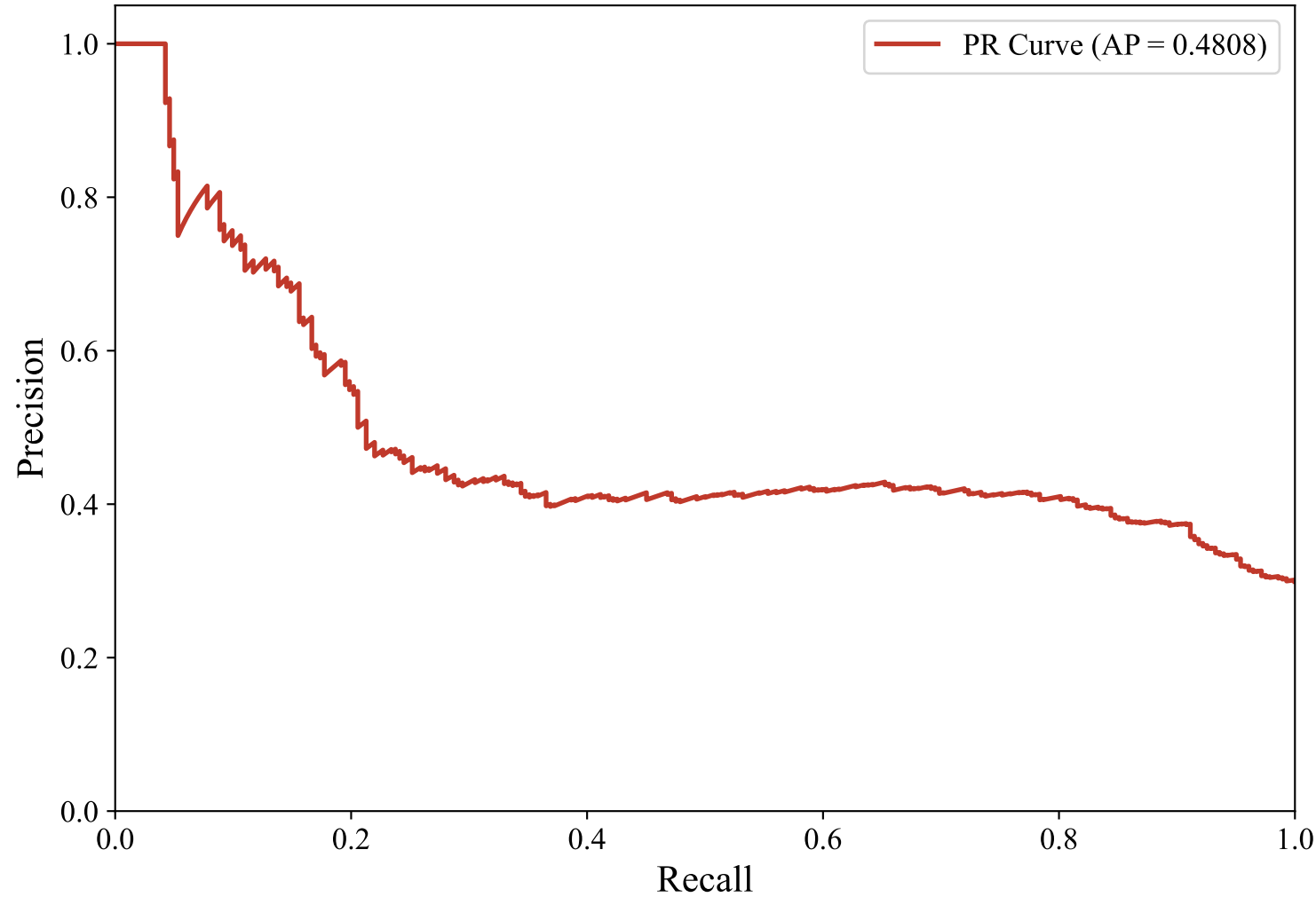
Precision-Recall Curve — ENGLISH_MANUAL (snowflake-arctic-embed-l-v2.0, lightgbm)
