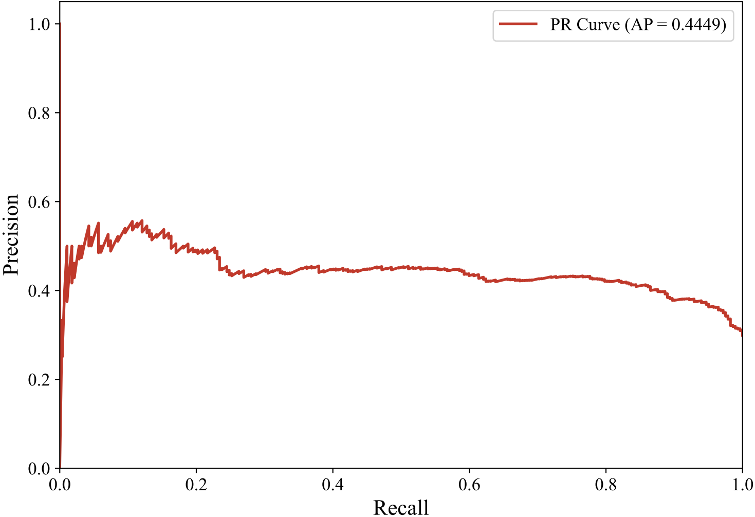
Precision-Recall Curve — ENGLISH_MANUAL (xlm-roberta-base, svm_linear)
