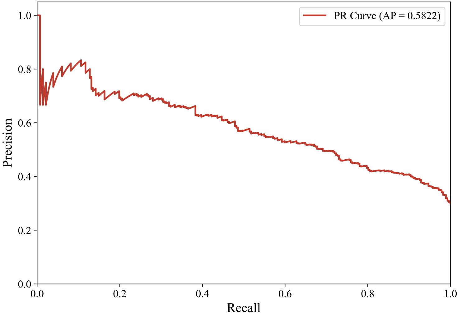
Precision-Recall Curve — ENGLISH_MANUAL (xlm-roberta-base, svm_rbf)
