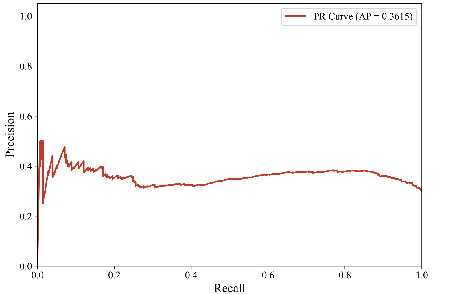
Precision-Recall Curve — ENGLISH_MANUAL (xlm-roberta-base, xgboost)
