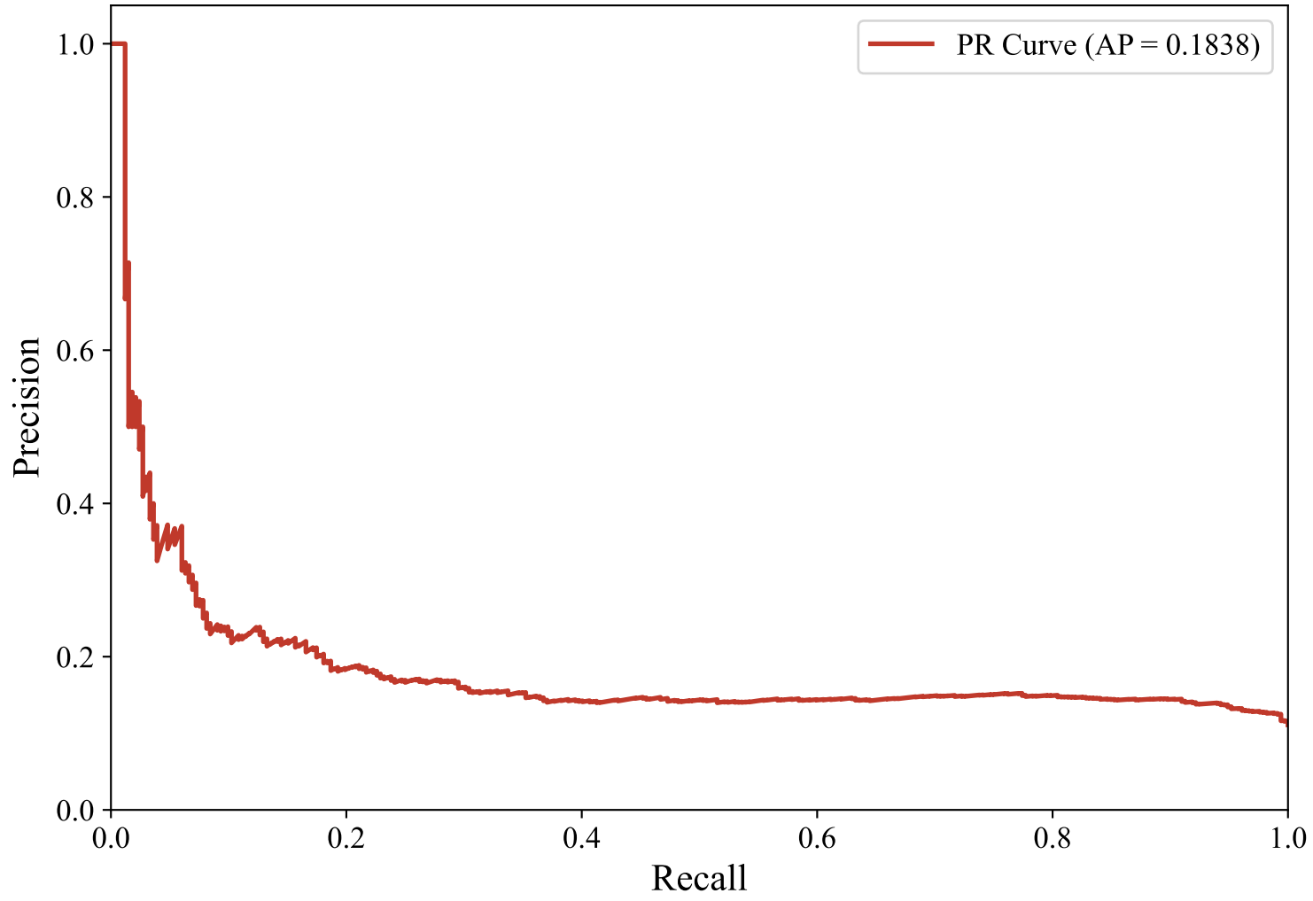
Precision-Recall Curve — GERMAN_MANUAL (multilingual-e5-large-instruct, lightgbm)
