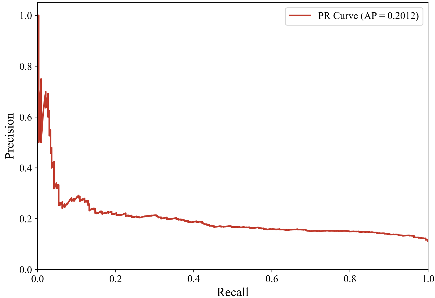
Precision-Recall Curve — GERMAN_MANUAL (multilingual-e5-large-instruct, random_forest)
