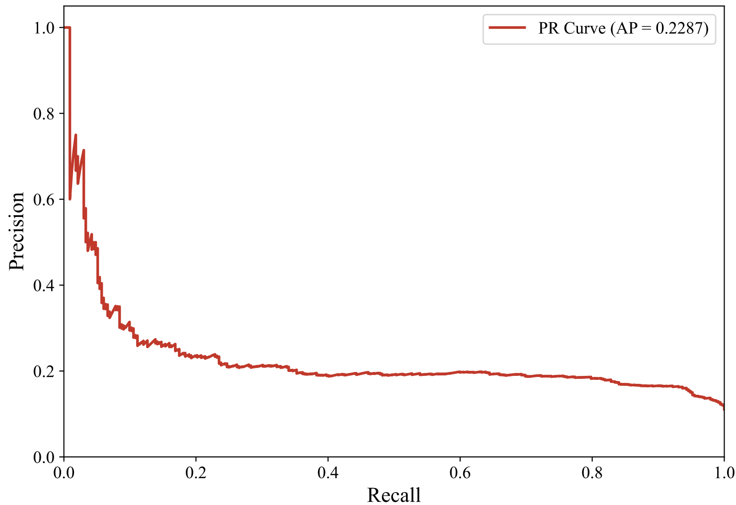
Precision-Recall Curve — GERMAN_MANUAL (multilingual-e5-large-instruct, svm_rbf)
