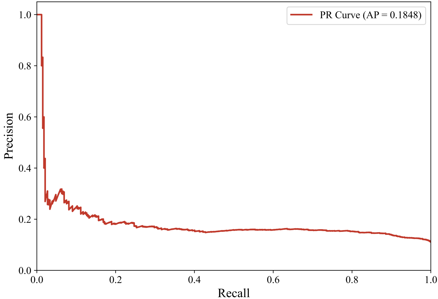
Precision-Recall Curve — GERMAN_MANUAL (paraphrase-multilingual-MiniLM-L12-v2, svm_linear)
